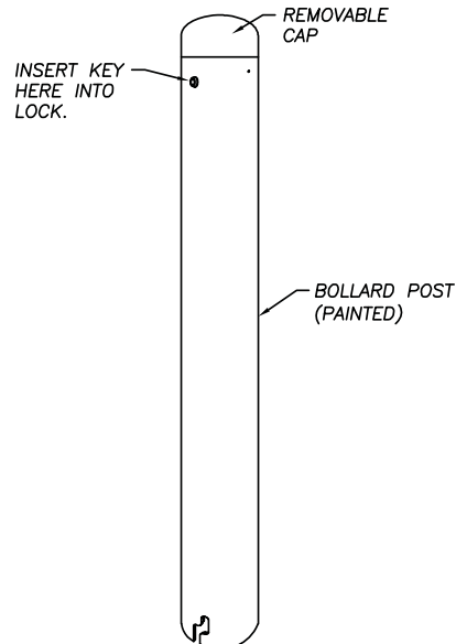
4.5" DIA. BOLLARD
